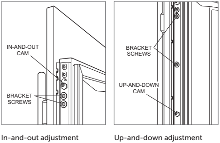
In-and-out adjustment
