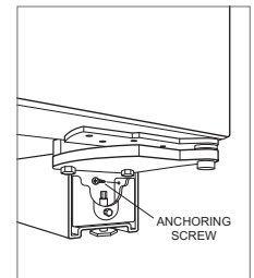
Bottom anchoring
