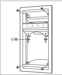
饮水机挡板拆卸
