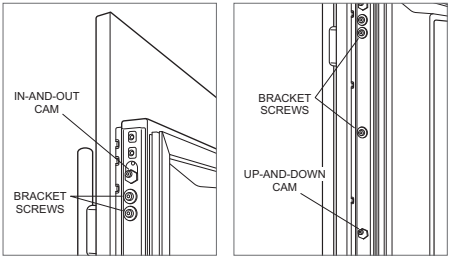
In-and-out adjustment Up-and-down adjustment
