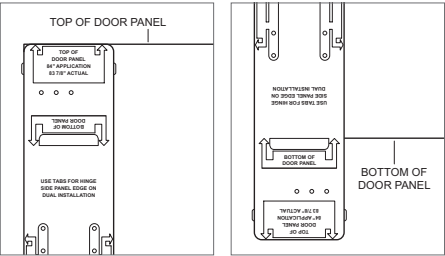
Door panel template—top Door panel template—bottom (tall models only)
