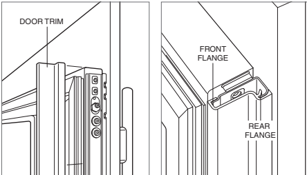
Door trim Bracket flanges
