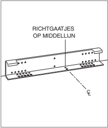
Anti-kantelbeugel
