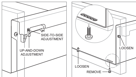
Drawer adjustment
