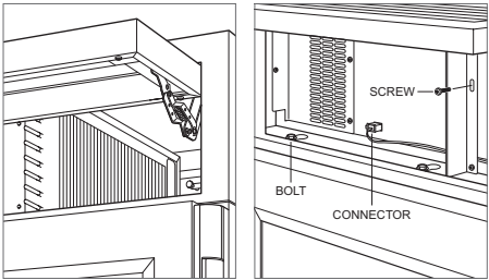
Lift grille
