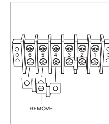
3-phase
